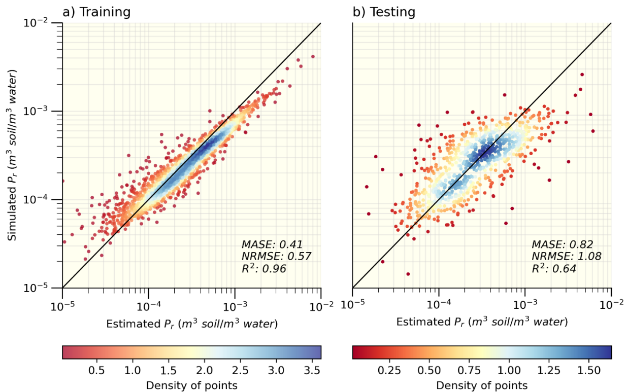
Figure S7. Performance of the XGBoost model with 15 predictors during a) the training phase (n=1816) and b) the testing phase (n=779). The solid black line indicates a 1:1 ratio. Note that the axes are in a log-log scale.
