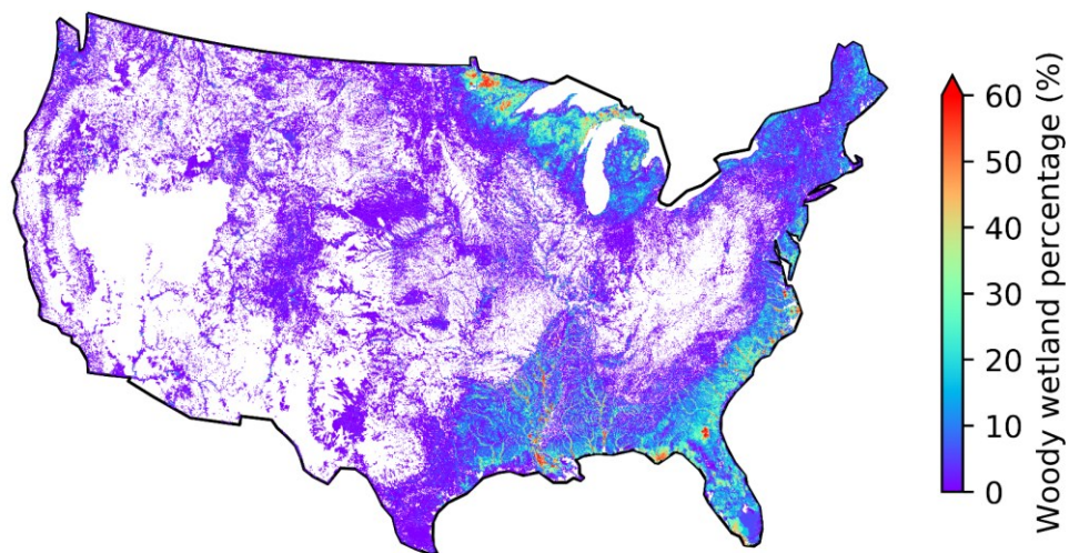
Figure S5. CONUS maps of: a) HWSO top-layer soil organic carbon (SOC) concentration, and b) woody wetland fraction across over 2 million NHDPlus catchments. Regions displayed in white may indicate missing data or a zero fraction.
