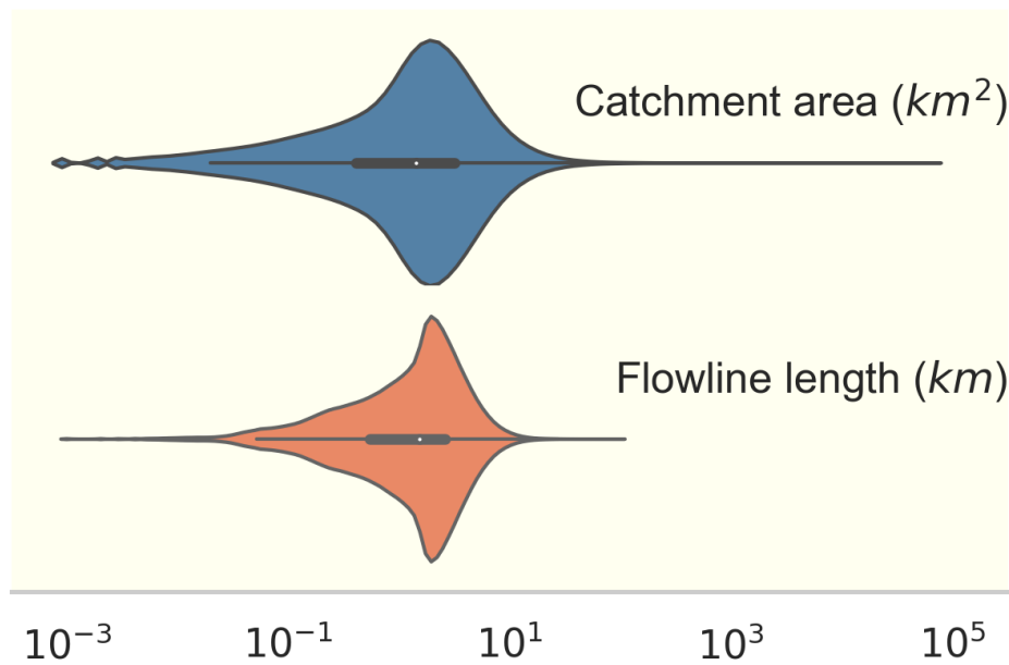
Figure S1. Distribution of the NHDPlus local catchment area and length of flowlines.
