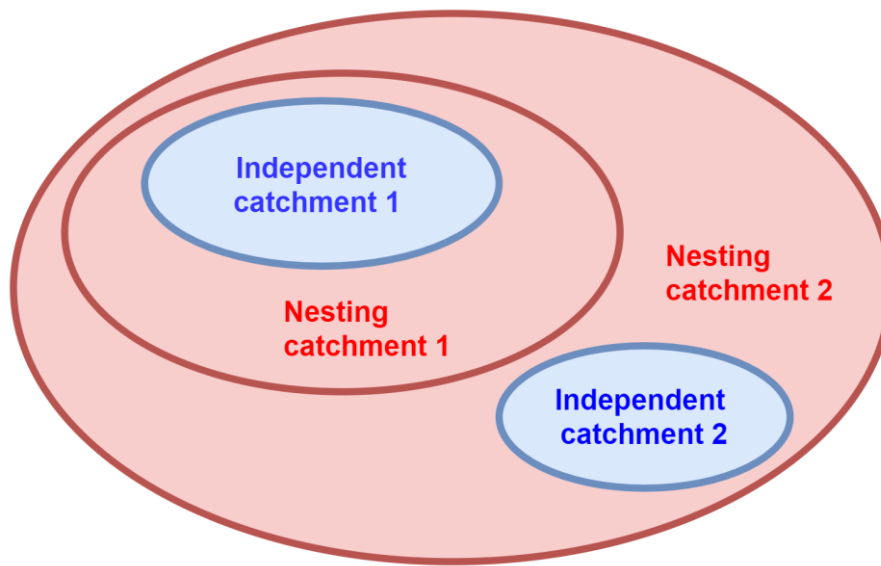
Figure S2. Conceptual diagram of identifying independent catchment.
