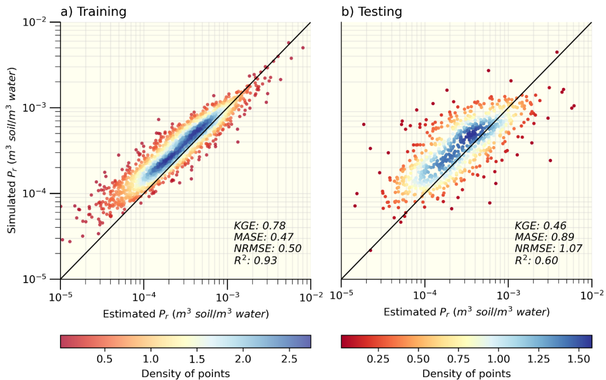
20 Figure S4. Performance of the XGBoost model with 12 predictors trained by using KGE during a) the training phase (n=1816) and b) the testing phase (n=779). The solid black line indicates a 1:1 ratio. Note that the axes are in a log-log scale.
