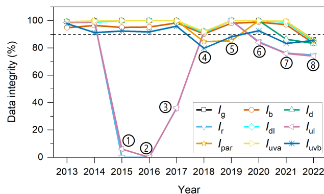
Figure 7. Data integrity of nine radiation components at the SDZ during the period 2013–2022.
