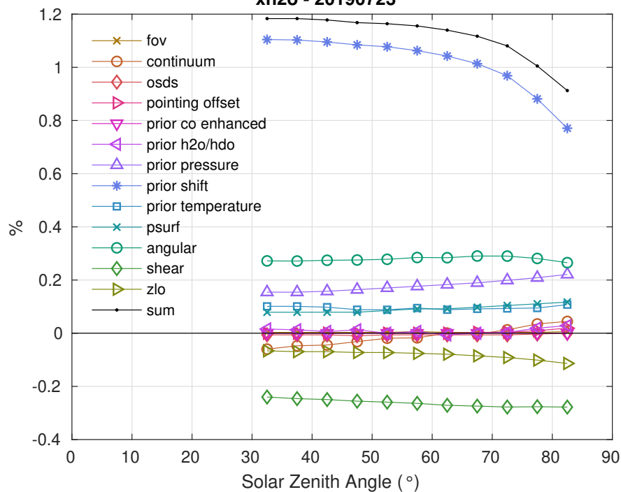
xn2o - 20190723
