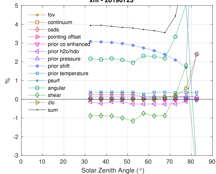
xhf - 20190723
