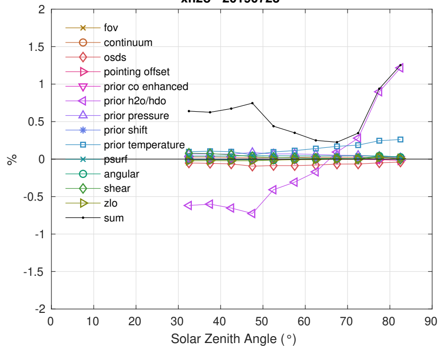
xh2o - 20190723
