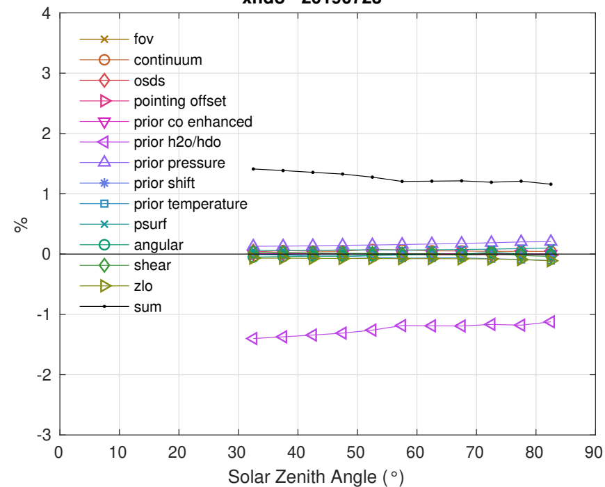
xhdo - 20190723
