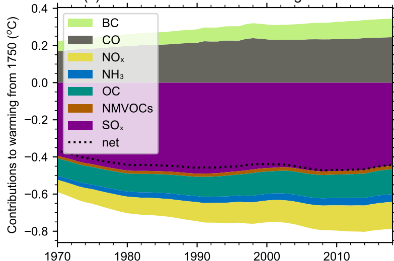
(c) SLCF contributions to warming from 1750
